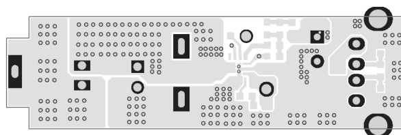
Figure 4: Bottom Layer
