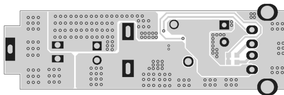
Figure 2: Top Layer
