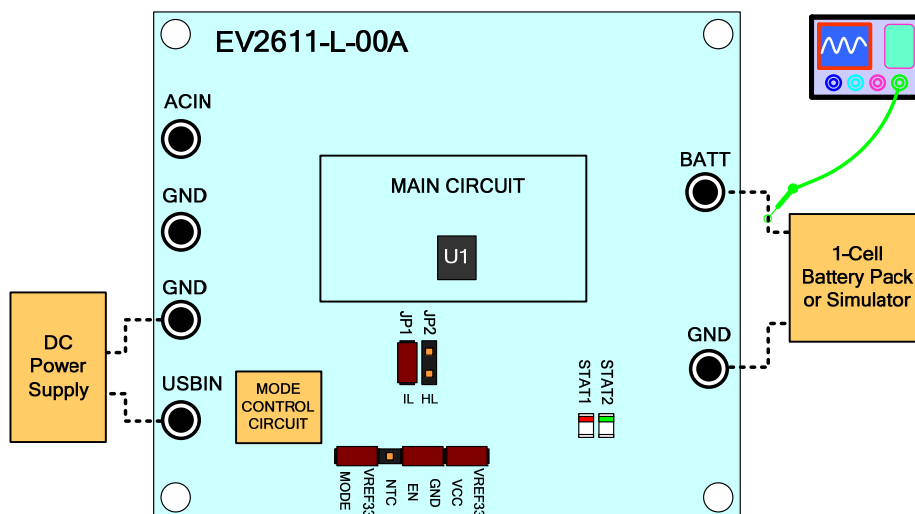
Figure 6—Setup for Single Input Application
