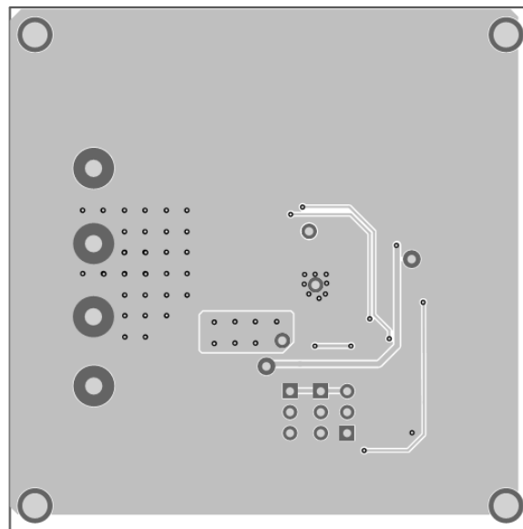
Figure 4: Bottom Layer
