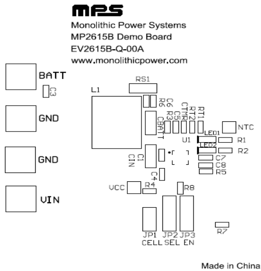
Figure 2: Top Silk
