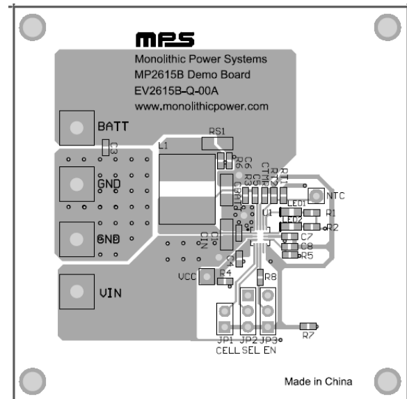
Figure 3: Top Layer
