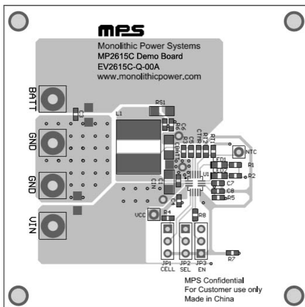
Figure 3: Top Layer
