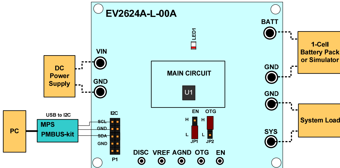
Figure1 Test Setup for MP2624A
