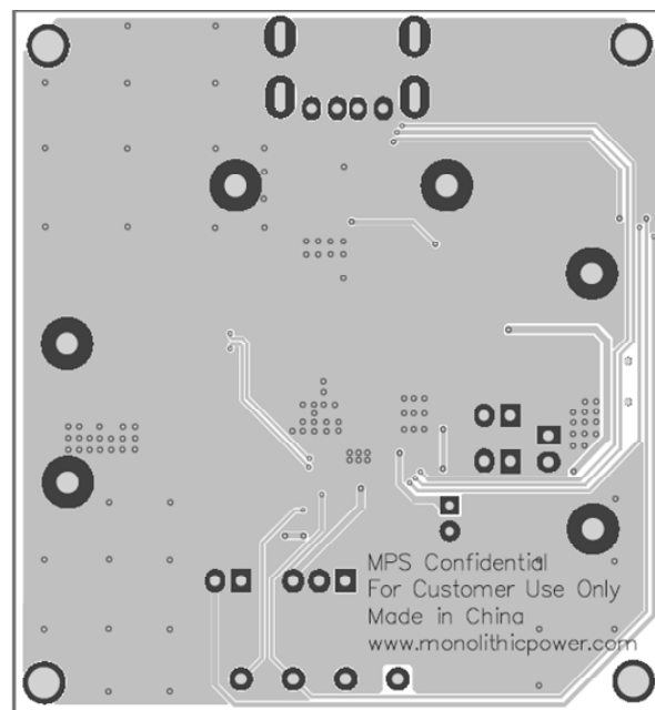
Figure 3: Bottom Layer
