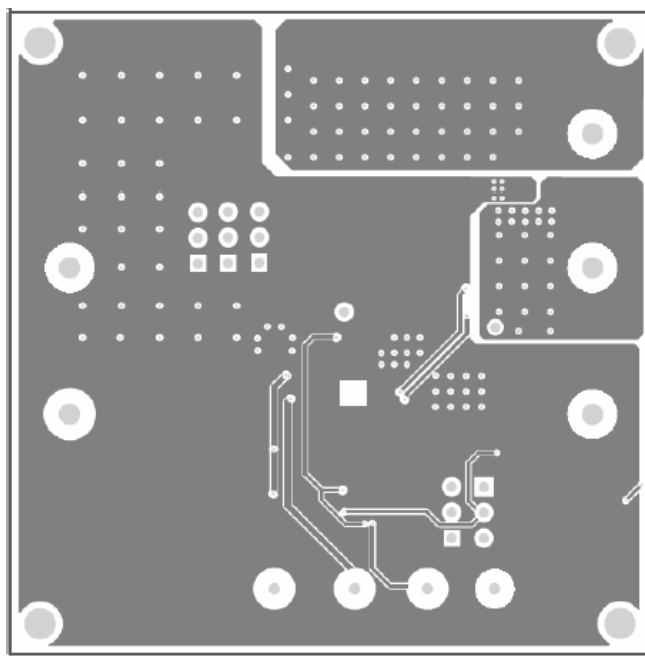
Figure 3: Bottom Layer
