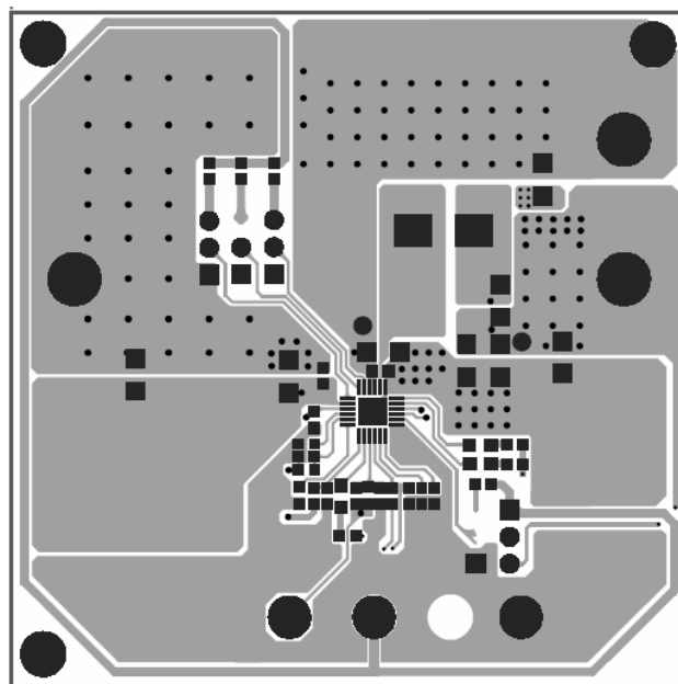
Figure 2: Top Layer
