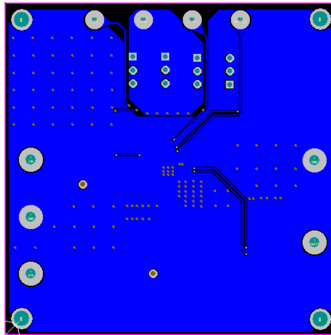
Figure 3: Bottom Layer
