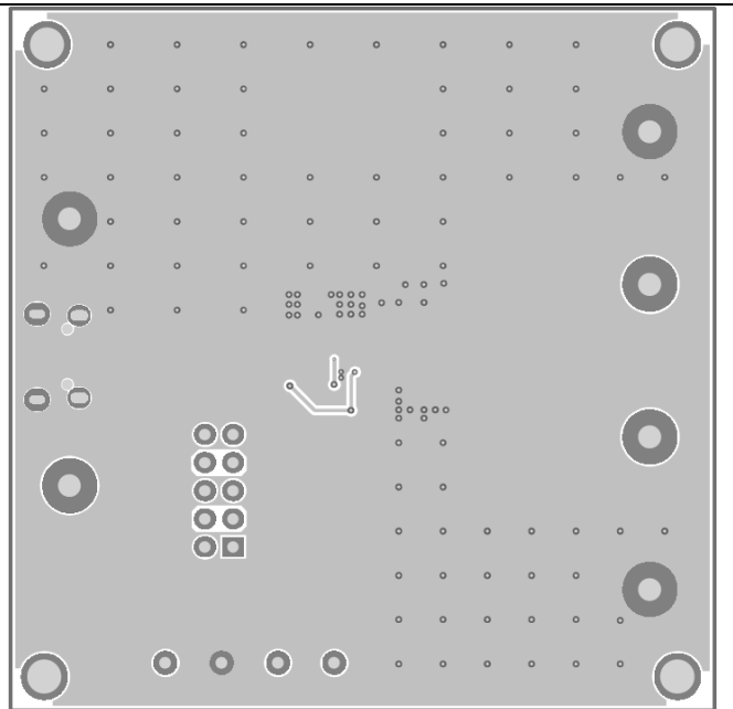
Figure 2: Bottom Layer
