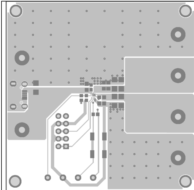
Figure 1: Top Layer
