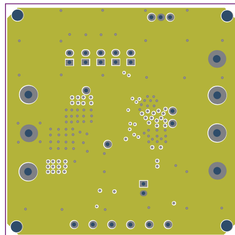
Figure 12: Mid-Layer 1
