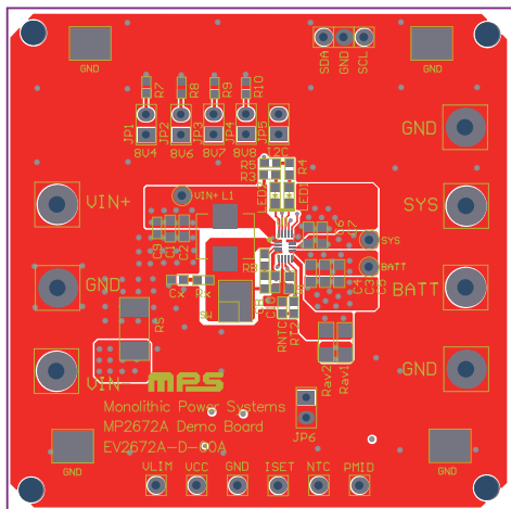
Figure 11: Top Layer
