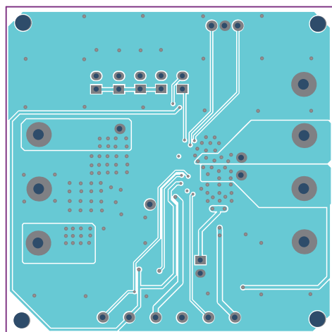
Figure 13: Mid-Layer 2
