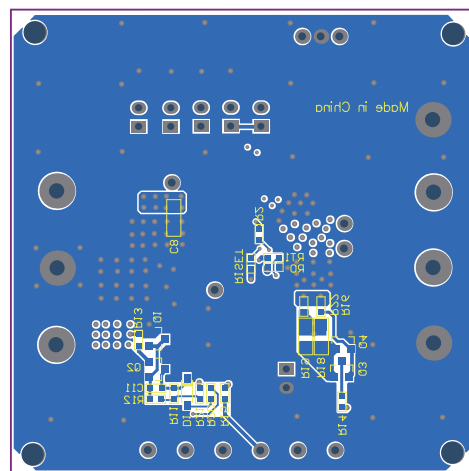
Figure 14: Bottom Layer
