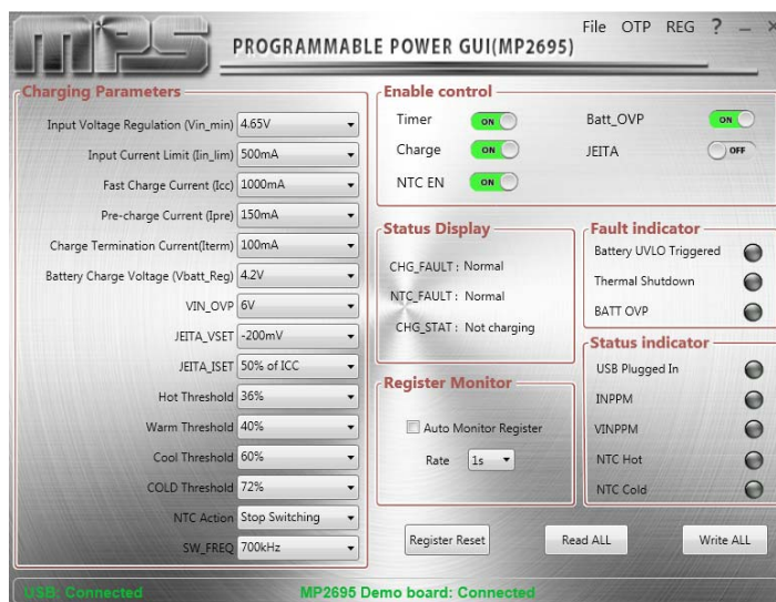
(2) normal connection
