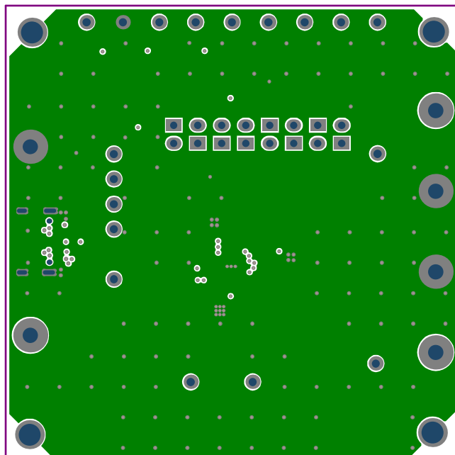
Figure 6: Mid-Layer 1
