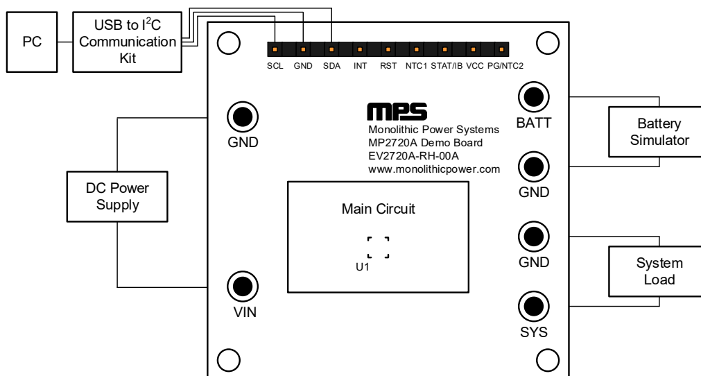
Figure 2: Measurement Equipment Set-Up
