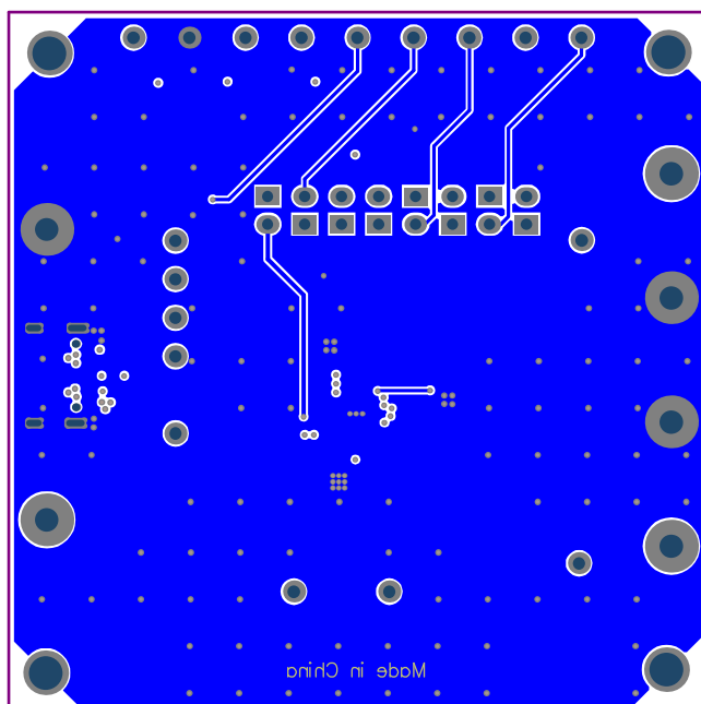
Figure 8: Bottom Layer
