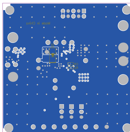
Figure 35: Bottom Layer
