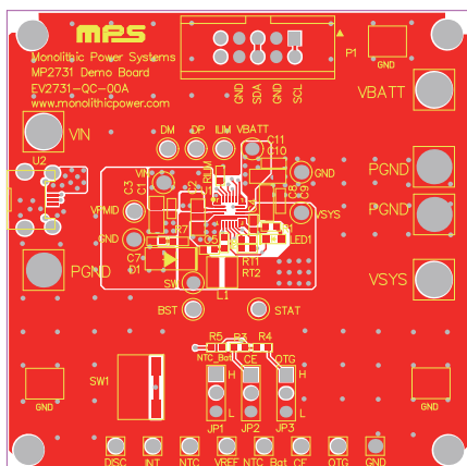
Figure 32: Top Layer
