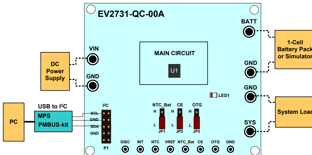
Figure 2: Test Set-Up for the MP2731
