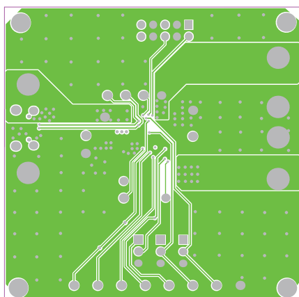
Figure 34: Mid-Layer 2
