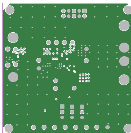
Figure 33: Mid-Layer 1
