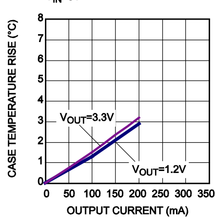
TRISING vs. Output Current V_{IN}=5V
