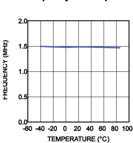
Frequency vs. Temperature
