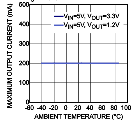
Output Current Derating vs. Ambient Temperature T_J \leq 125^\circ C
