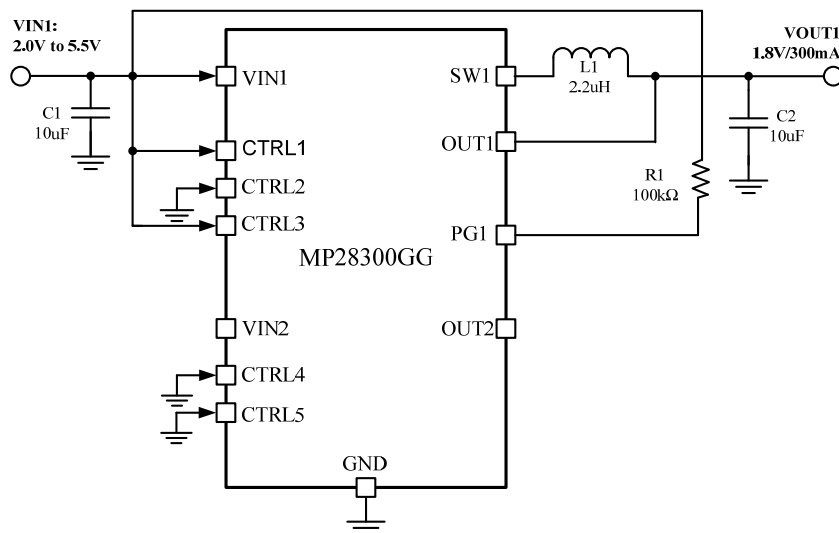
Figure 3—Typical Application Circuit only for Buck
