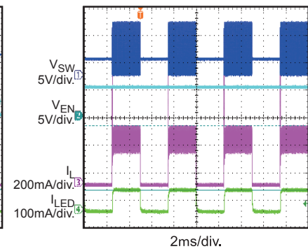
PWM Dimming
