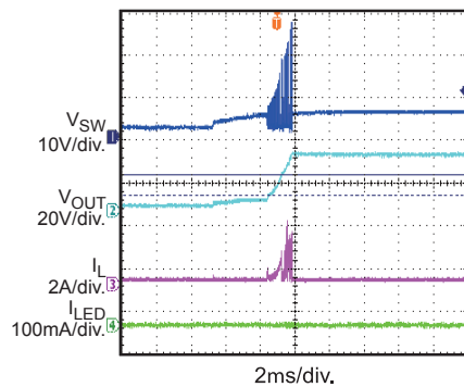
Start-Up when Open Load
