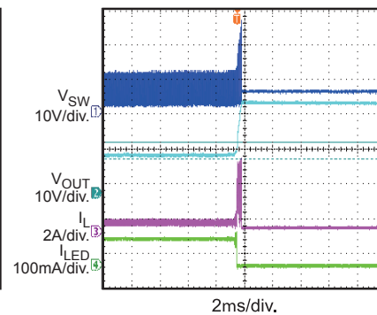
Open Load when Work Normal
