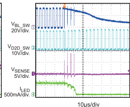
Short Diode
