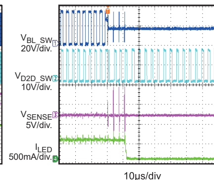
Short Inductor
