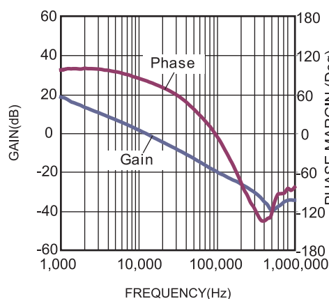
Bode Plot
