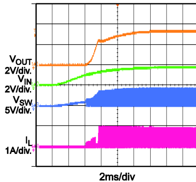
V_{IN} Startup
