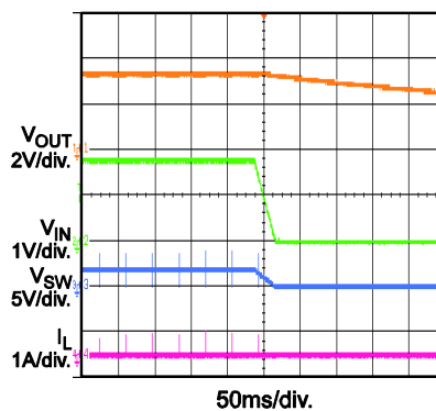
V_{IN} Shutdown
