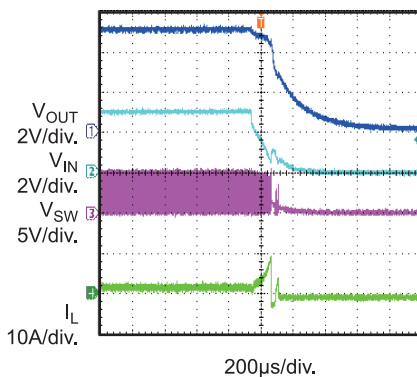
V_{IN} Shutdown
