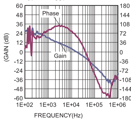
Bode Plot
