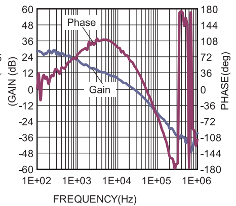
Bode Plot
