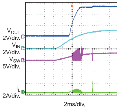
V_{IN} Startup
