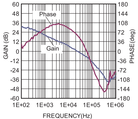
Bode Plot
