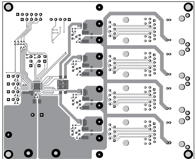
Figure 2: Top Layer
