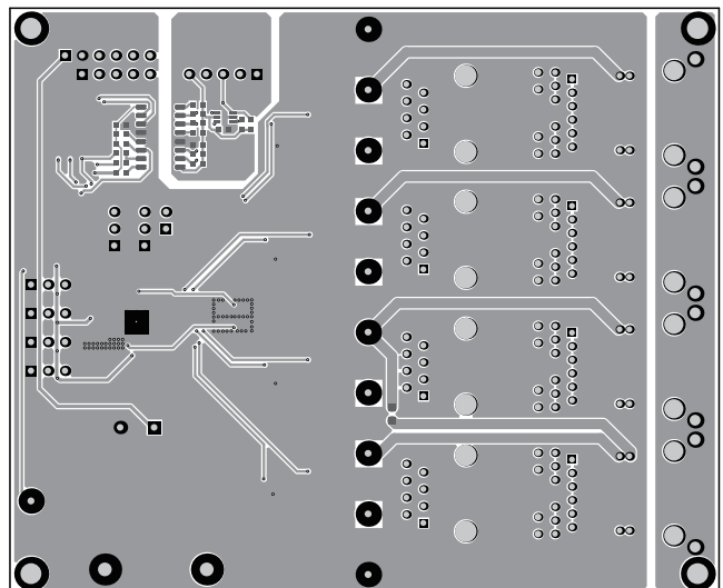
Figure 4: Bottom Layer
