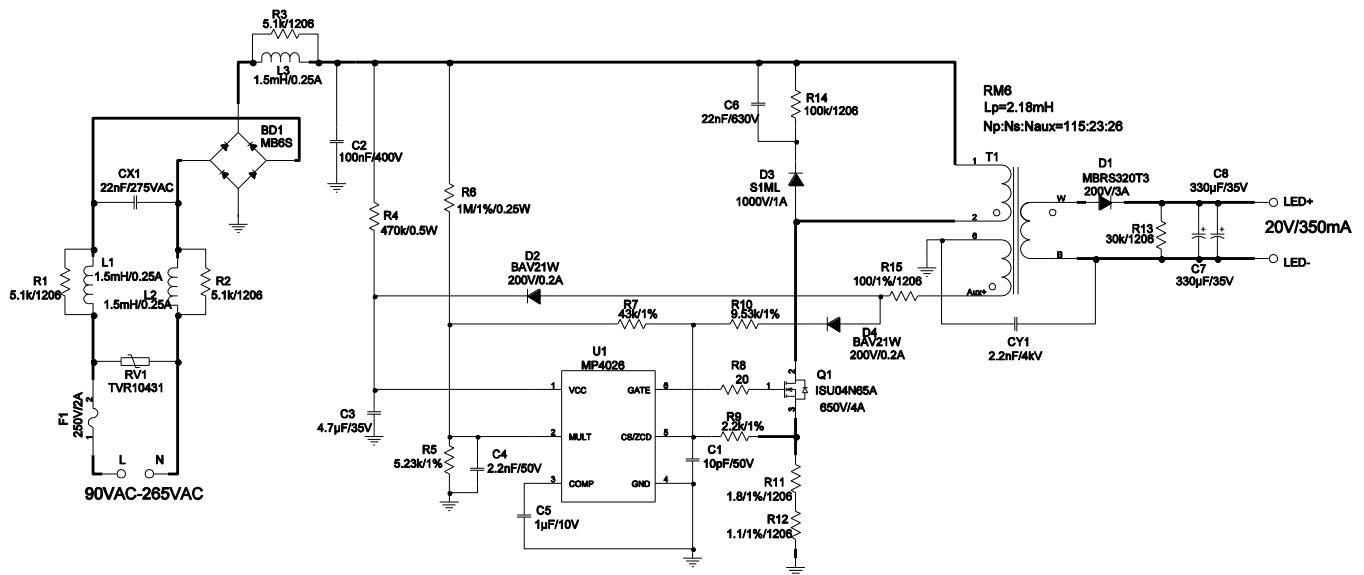
Figure 1 - Schematic
