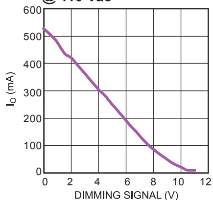
Analog Dimming Curve @ 110 Vac
