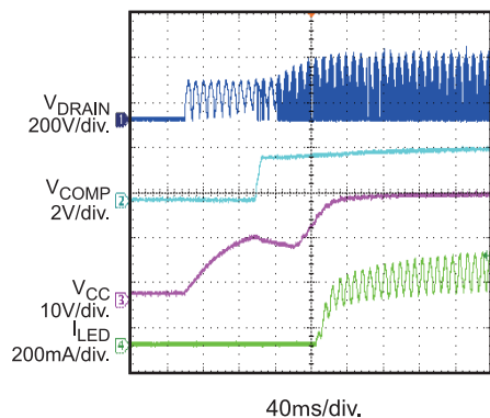
V_{IN} Start-Up
