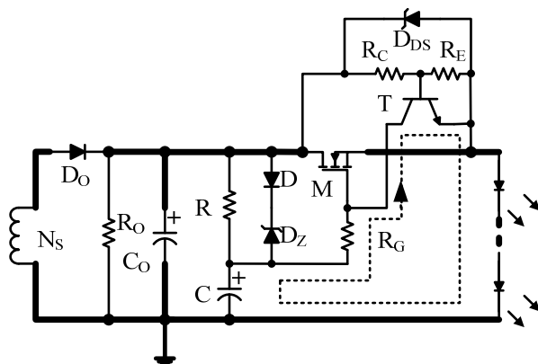
Figure 8—Drain-Source OVP and OCP Circuit
