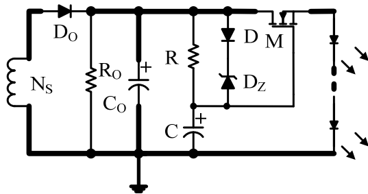
Figure6—Ripple Suppressor
