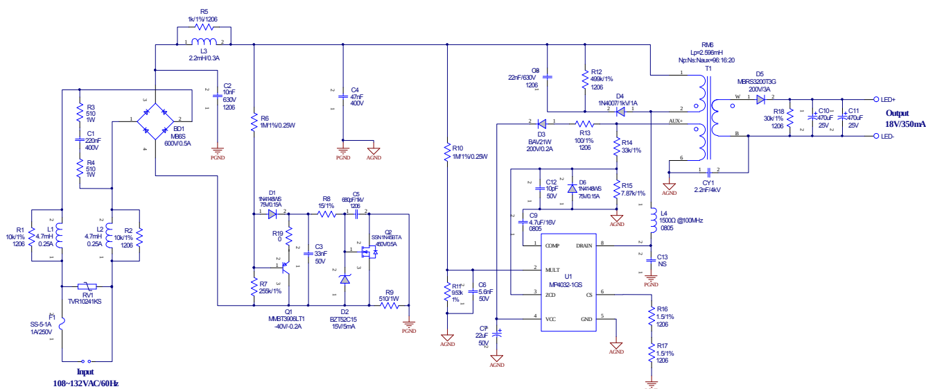
Figure 1—Schematic
