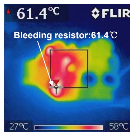
50% dimming @ Vin=120V AC
