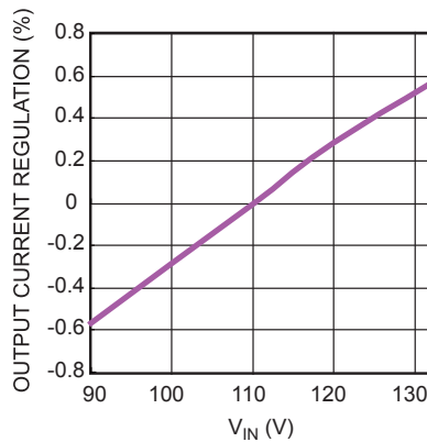
Line Regulation
