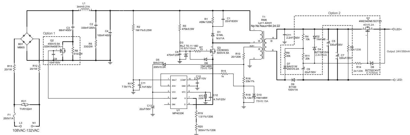
Figure 1—Schematic
