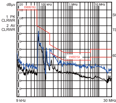
Conducted EMI N-Line
