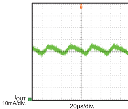
Output Current Ripple
