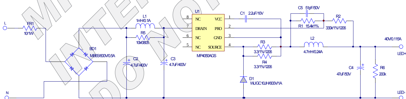
Figure 1—Schematic
