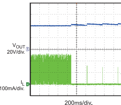
Open LED Protection Entry
