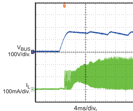
Soft Start
