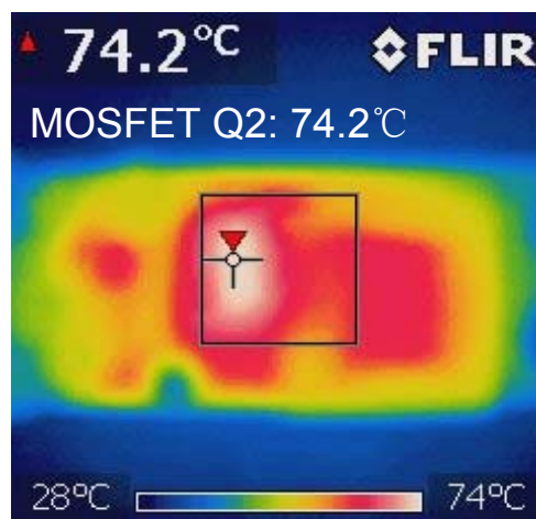
Trailing edge dimmer with 90% turn on phase
