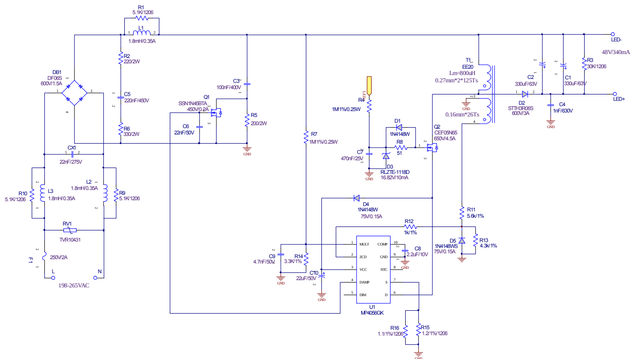
Figure 1—Schematic
