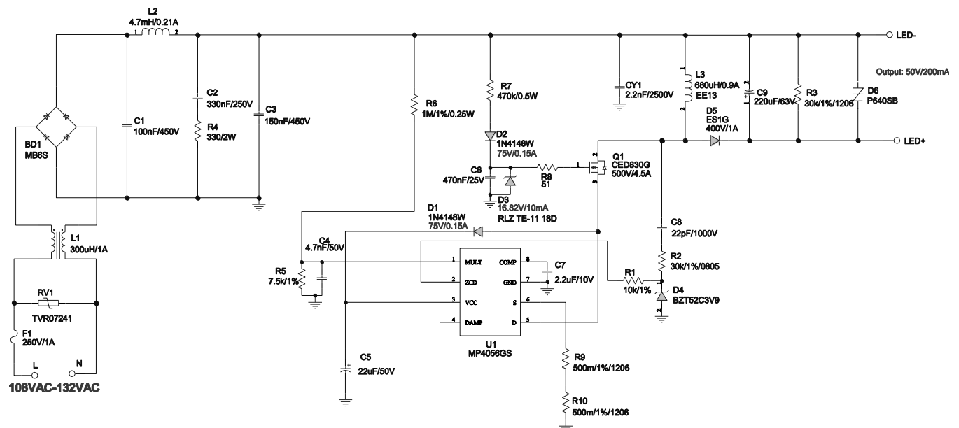
Figure 1—Schematic
