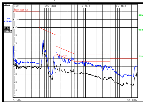
Conduct EMI-N Line V_{IN}=230Vac , 7 LED Output
