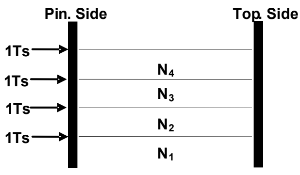
Figure 4—Winding Diagram
