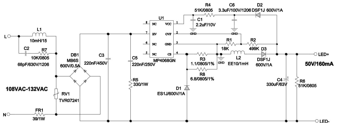
Figure 1—Schematic
