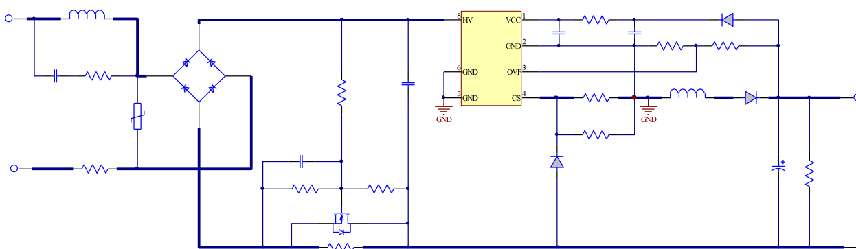
Figure 1—Schematic
