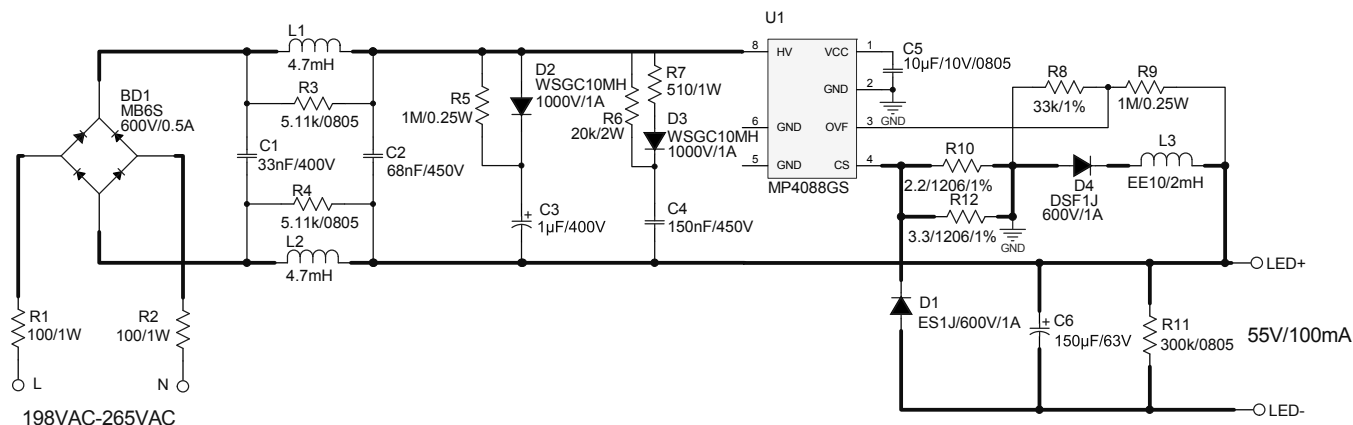
Figure 1—Schematic
