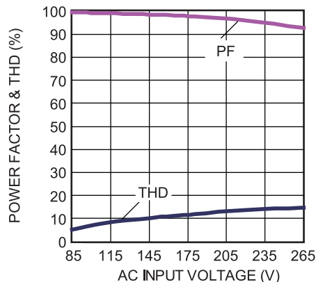
PF & THD vs. V_{AC}
