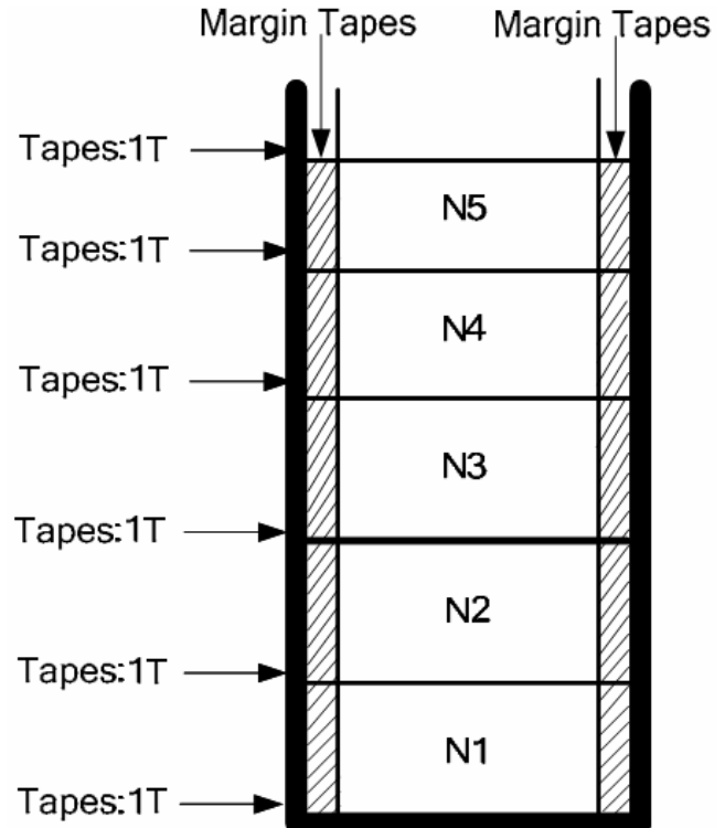
Winding Diagram
