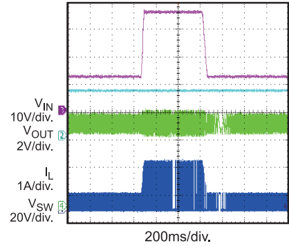
Load Dump
