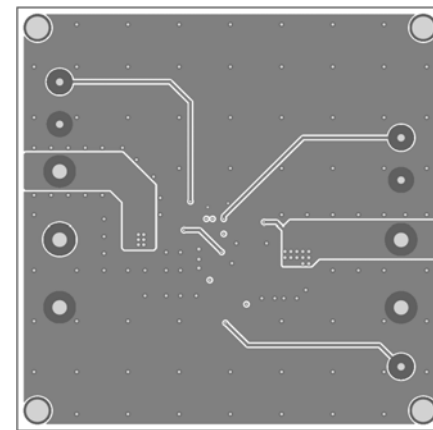
Figure 4 – Inner Layer 2
