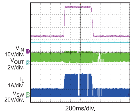
Load Dump
