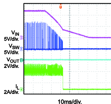
LED+ Short to GND Input Power Off
