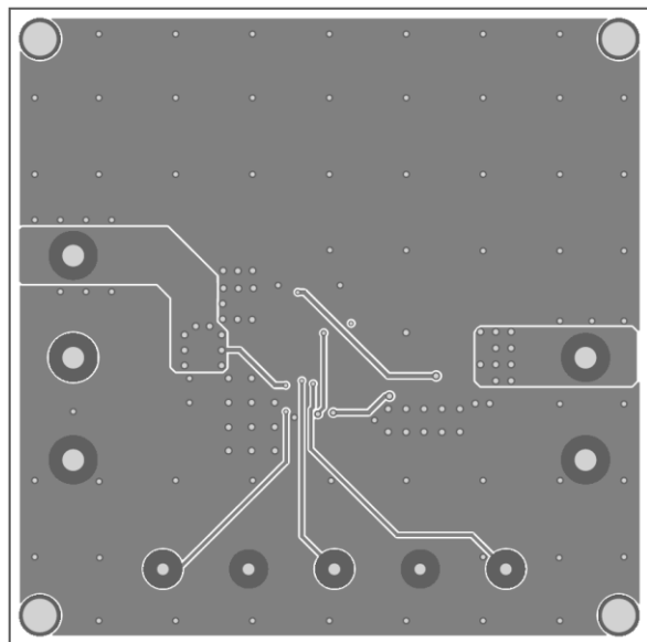
Figure 3—Inner2 Layer
