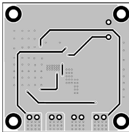
Figure 4—Inner Layer 2
