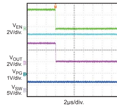
Power Good Through EN Shutdown
