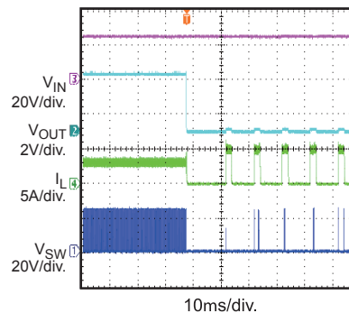
Short Circuit Recovery
