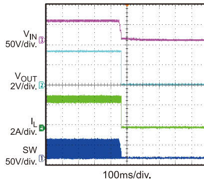
Shutdonw Through V_{IN}
