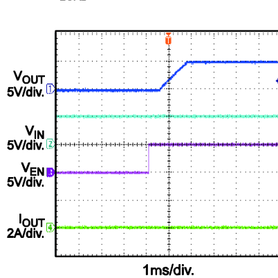
Start-Up through Enable I_{LOAD}=0A
