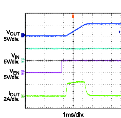
Start-Up through Enable I_{LOAD}=0A , C_{OUT}=1000\mu F
