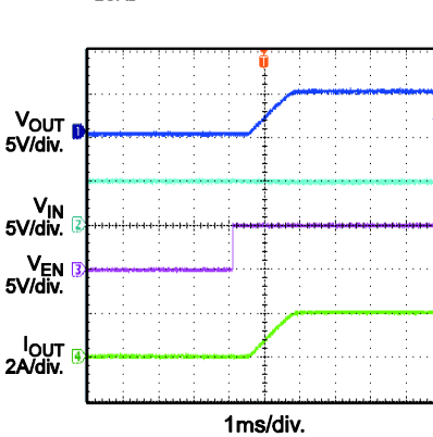
Start-Up through Enable I_{LOAD}=2A
