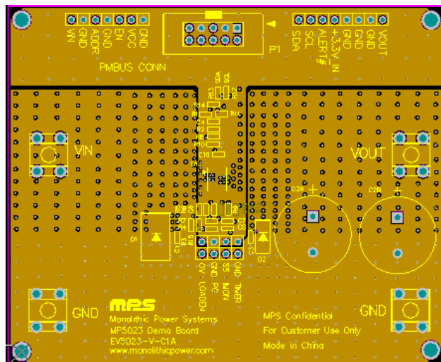
Figure 2—Inner Layer1
