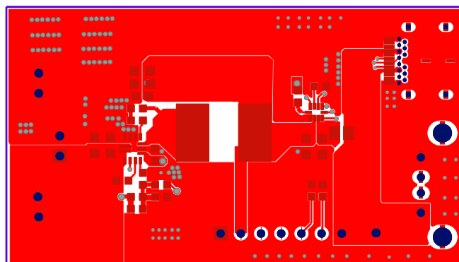
Figure 2: Top Layer
