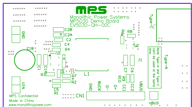
Figure 1: Top Silkscreen Layer
