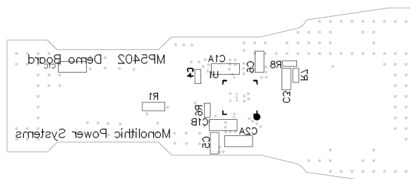
Figure 5—Bottom Silk Layer
