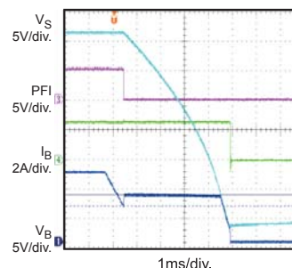
VSTRG Release P_B=20W , C_{STRG}=150\mu F
