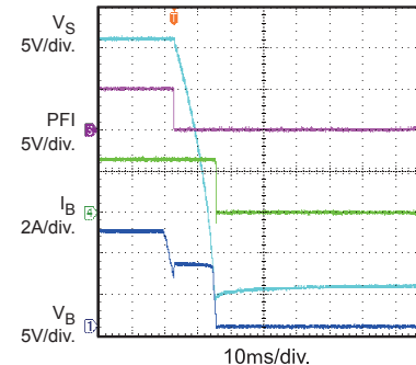
V_{STRG} Release
