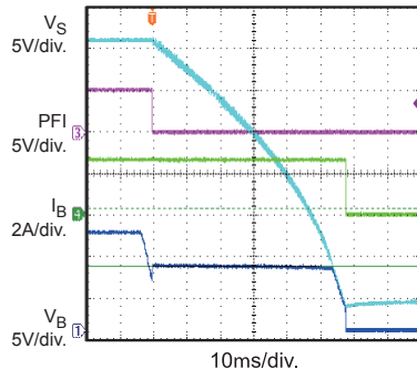
V_{STRG} Release
