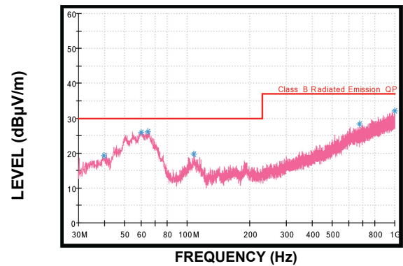
Radiated Emission Results (3)
