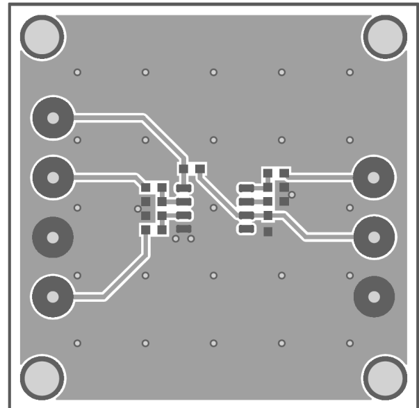
Figure 2: Top Layer
