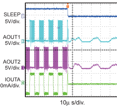
Sleep Entry (Full Step) V_{IN} = 9\text{V}
