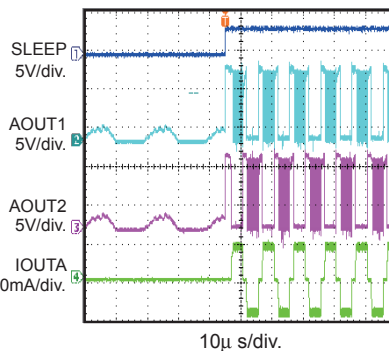
Sleep Recovery (Half-Step) V_{IN} = 9\text{V}
