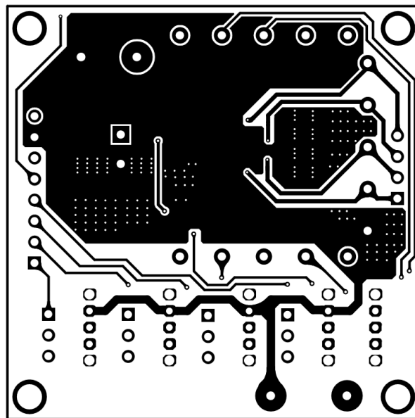
Figure 4: Bottom Layer
